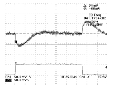
3.3V Transient Response
